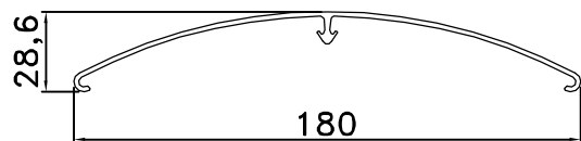
CA 180 PERIMETRE EXTERIEUR = 431mm
