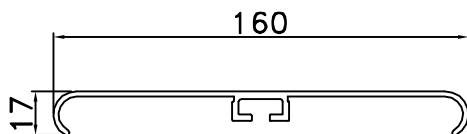
CA 160 PERIMETRE EXTERIEUR = 431mm
