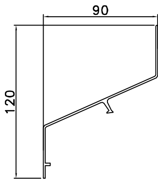
lame FL1200 PERIMETRE EXTERIEUR = 409mm
